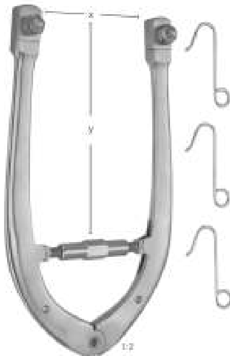
Kirschner Extension Bows 10-1472 x=180\text{mm} y=100\text{mm} 10-1473 x=270\text{mm} y=160\text{mm} with 3 traction hooks
